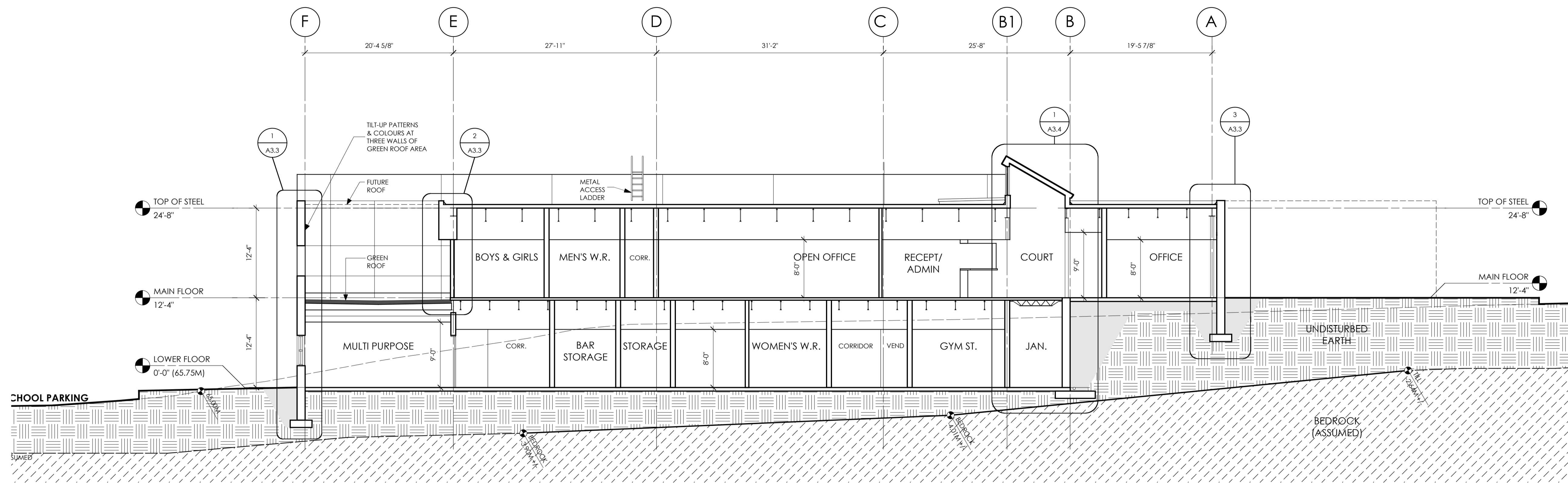
1 SECTION: BUILDING A1.1 1/8" = 1'-0"
