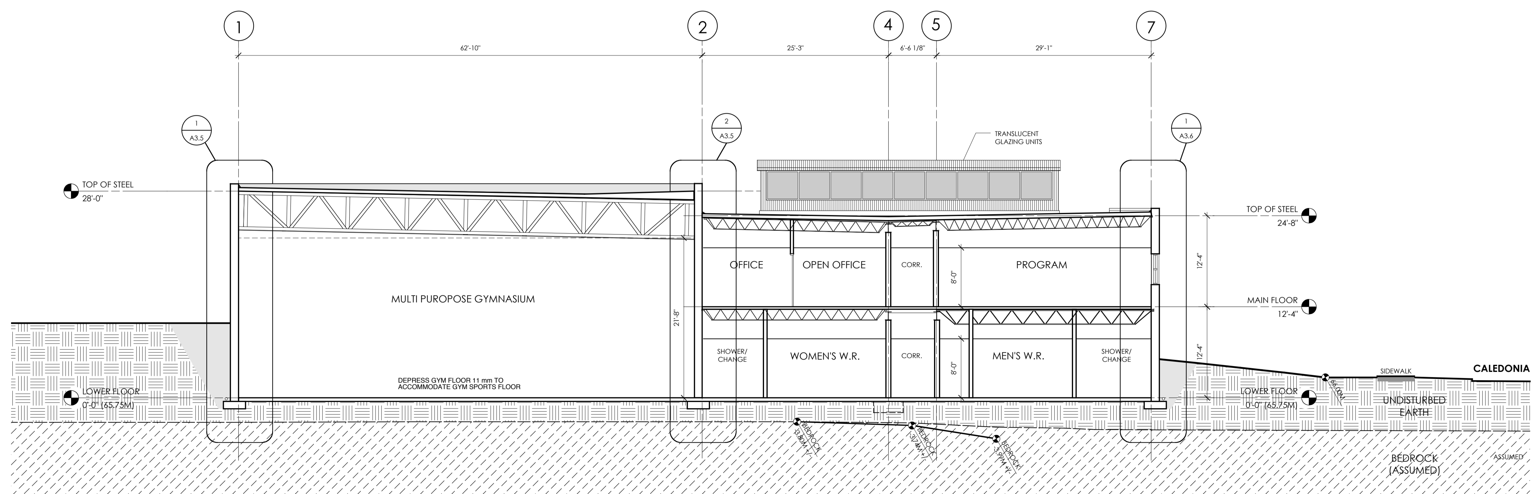
2 SECTION: BUILDING A1.1 1/8" = 1'-0"
