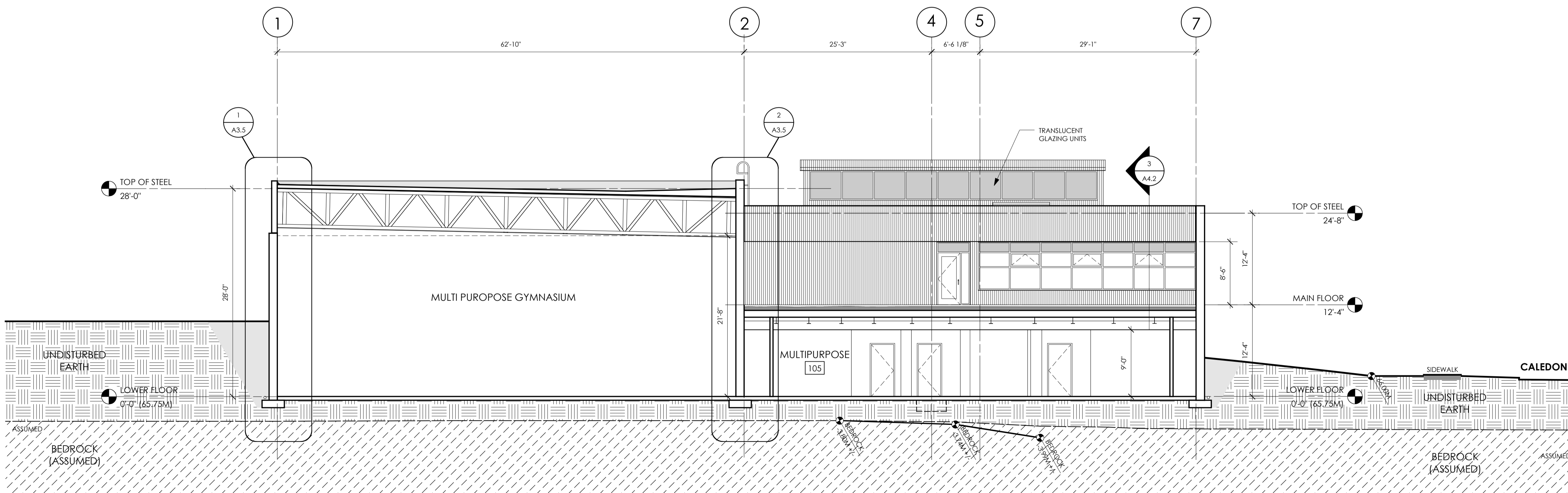
2 SECTION: BUILDING A1.1 1/8" = 1'-0"
