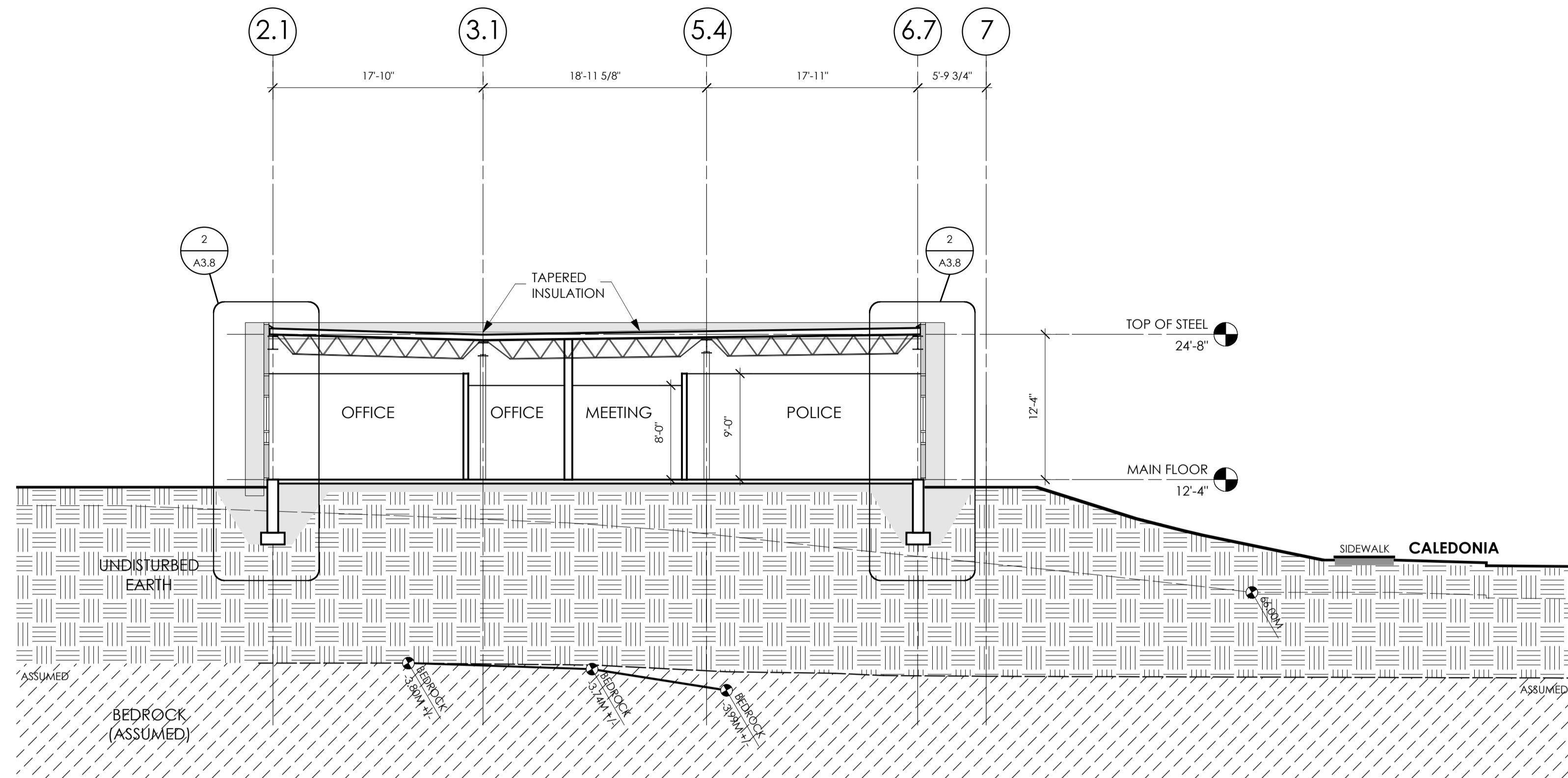
1 SECTION: BUILDING A1.2 1/8" = 1'-0"
