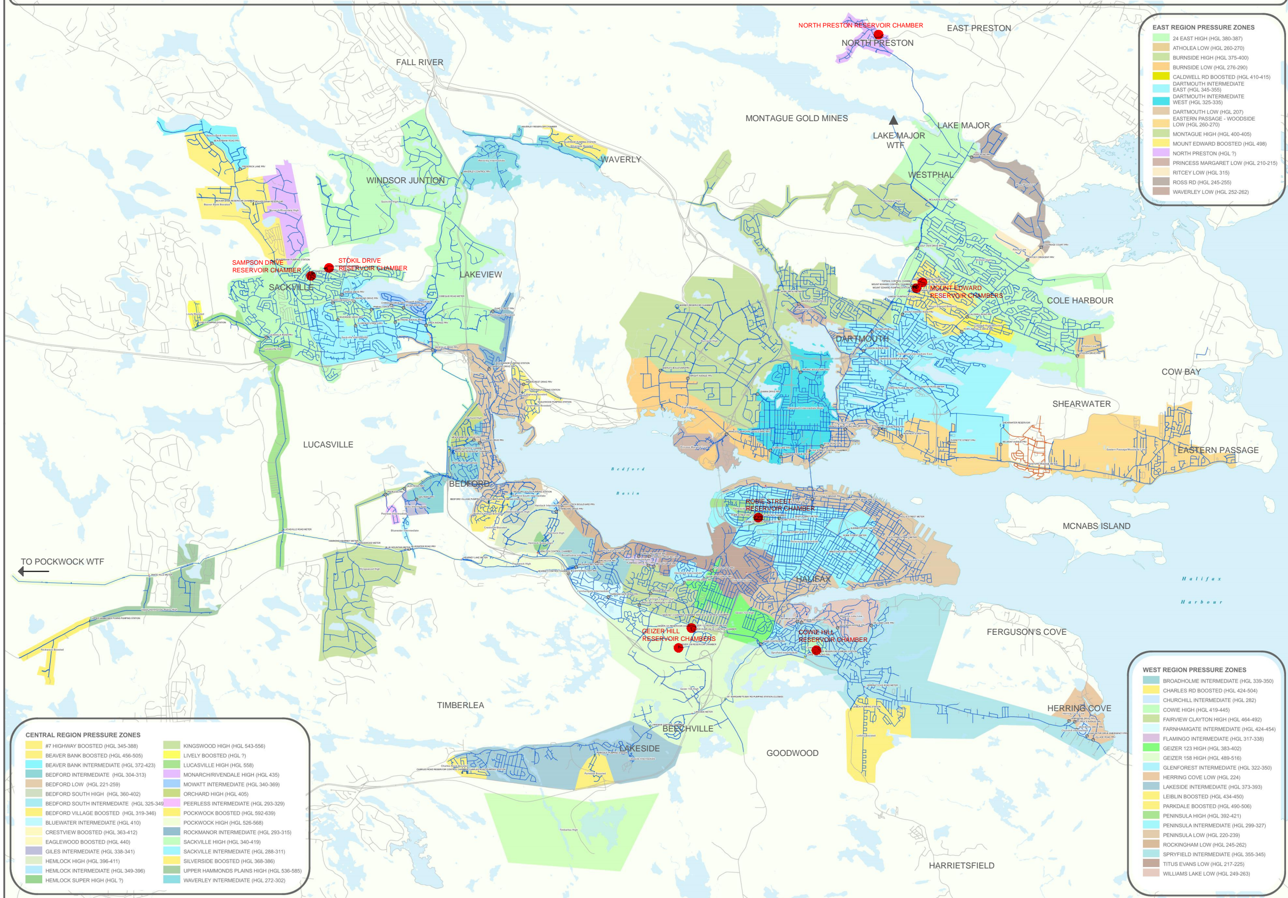
FIGURE 2.2 EXISTING WATER SYSTEM SCHEMATIC
