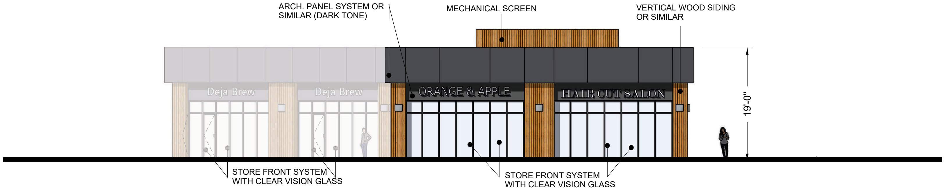
NORTHEAST ELEVATION
