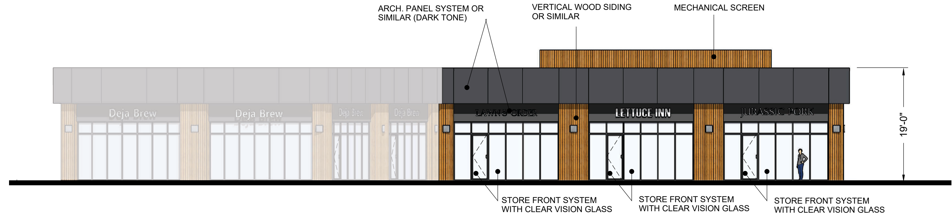
SOUTHEAST ELEVATION
