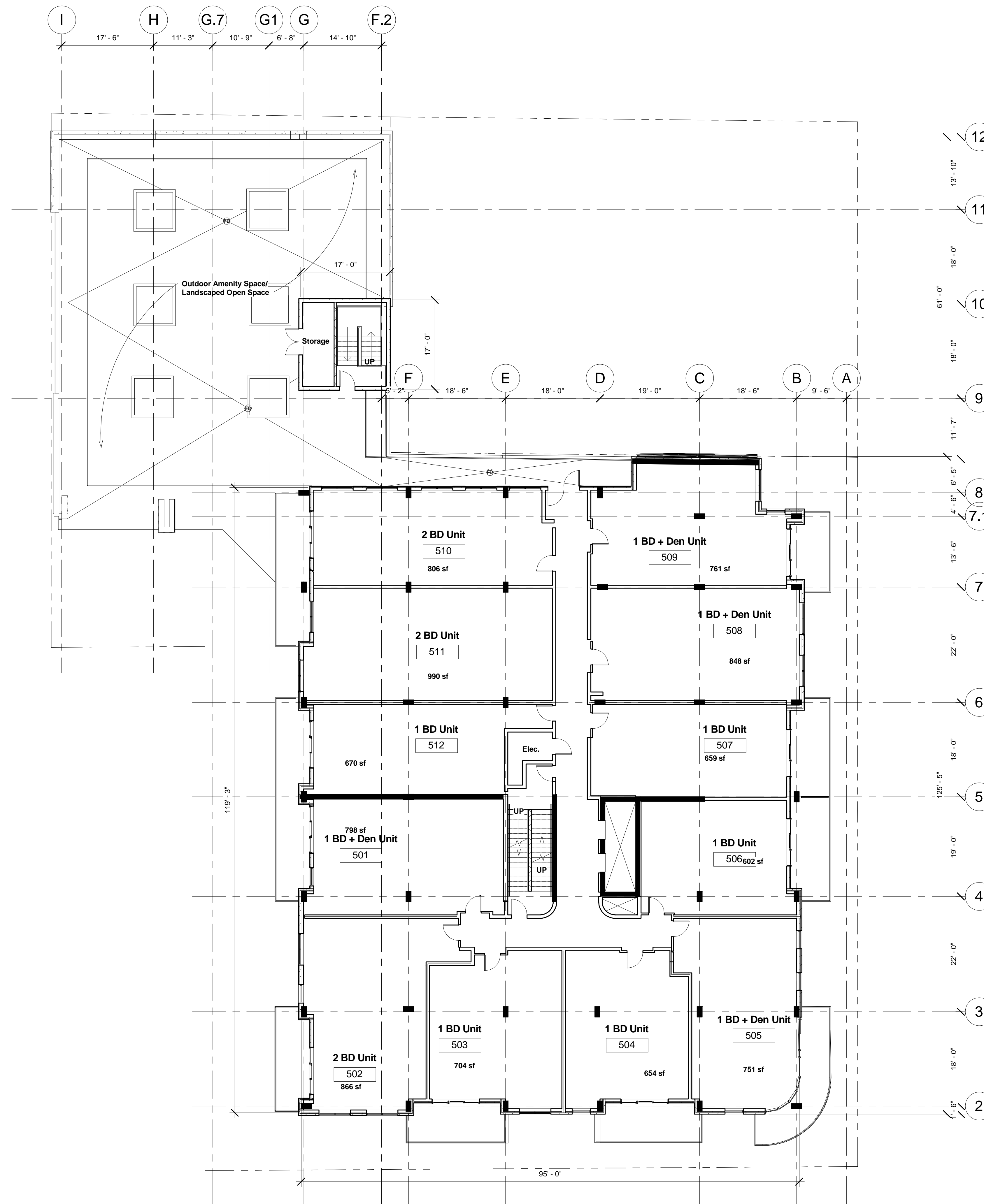
1 Level 5 DA 3/32" = 1'-0"
